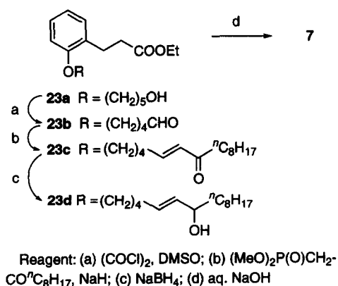
Scheme 5. Synthesis of compound 7.
