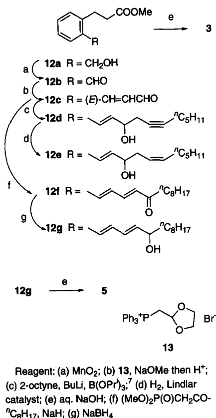
Scheme 2. Synthesis of compounds 3 and 5 .
