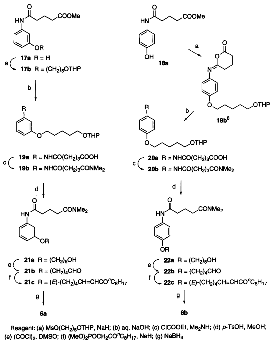
Scheme 4. Synthesis of compounds 6a–b.
