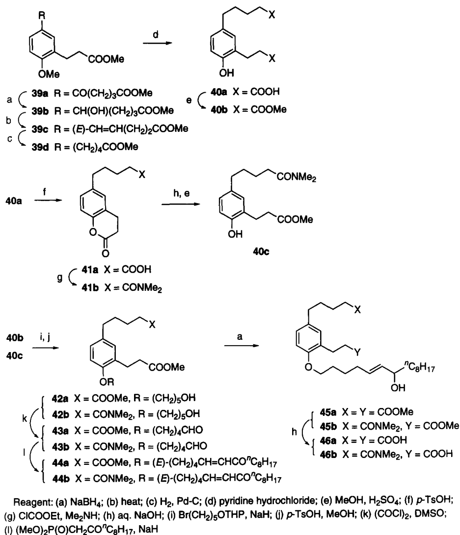
Scheme 9. Synthesis of compounds 46a–b.
