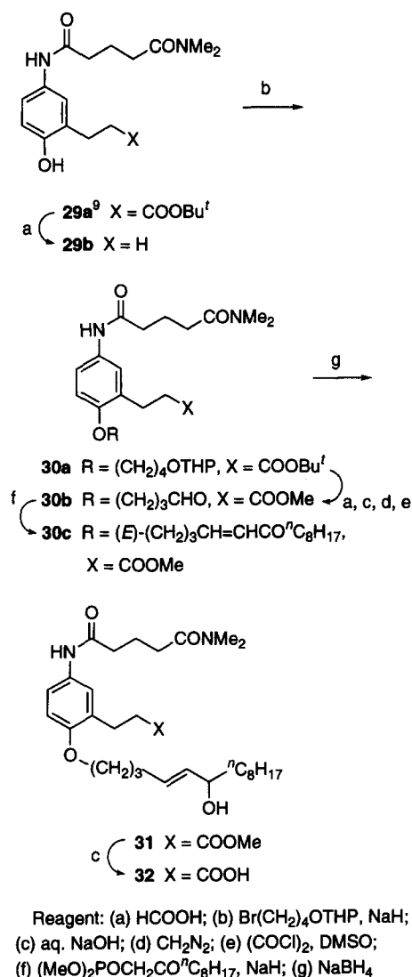
Scheme 7. Synthesis of compound 32.
