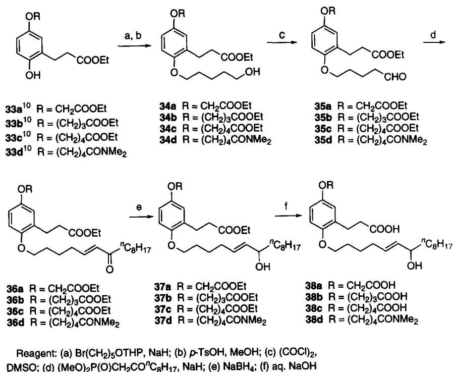
Scheme 8. Synthesis of compounds 38a–d.
