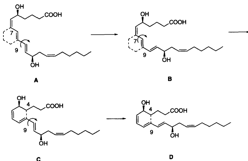
Chart 1. Possible conformers of LTB 4 (1).
