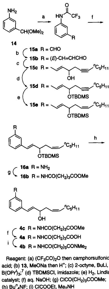
Scheme 3. Synthesis of compounds 4b–c .
