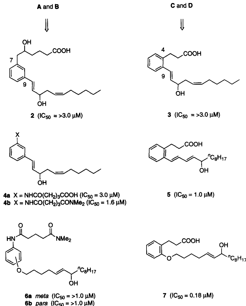
Chart 2. Partial fixation of conformers A–D.
