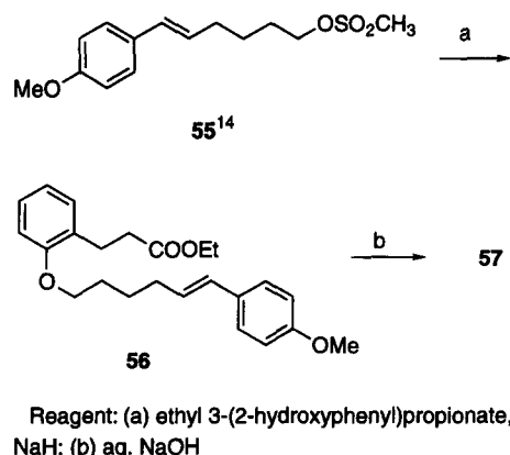
Scheme 12. Synthesis of compound 57 .
