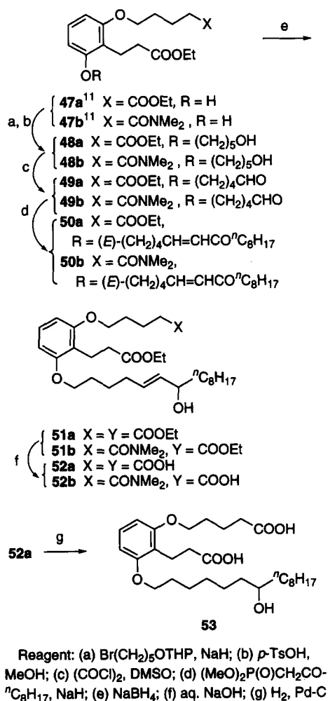
Scheme 10. Synthesis of compounds 52a–b and 53.
